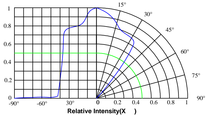
Fig.6 Radiation Diagram
