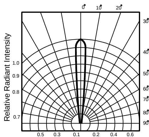
Fig.6 Radiation Diagram
